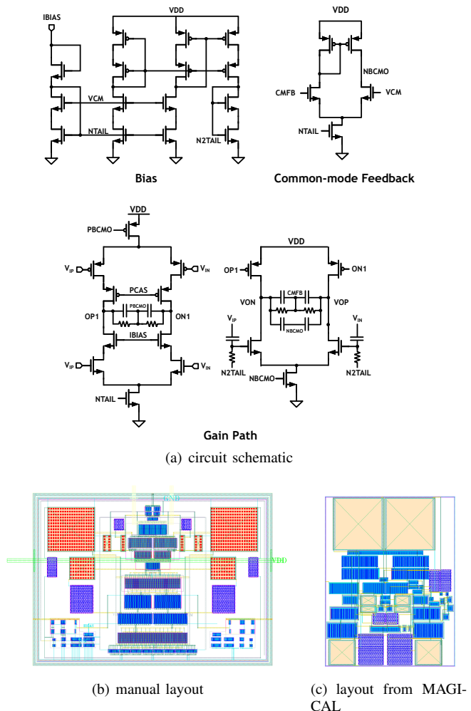
Fig. 7. Inverter-based OTA circuit schematic, manual layout, and layout result from MAGICAL.
